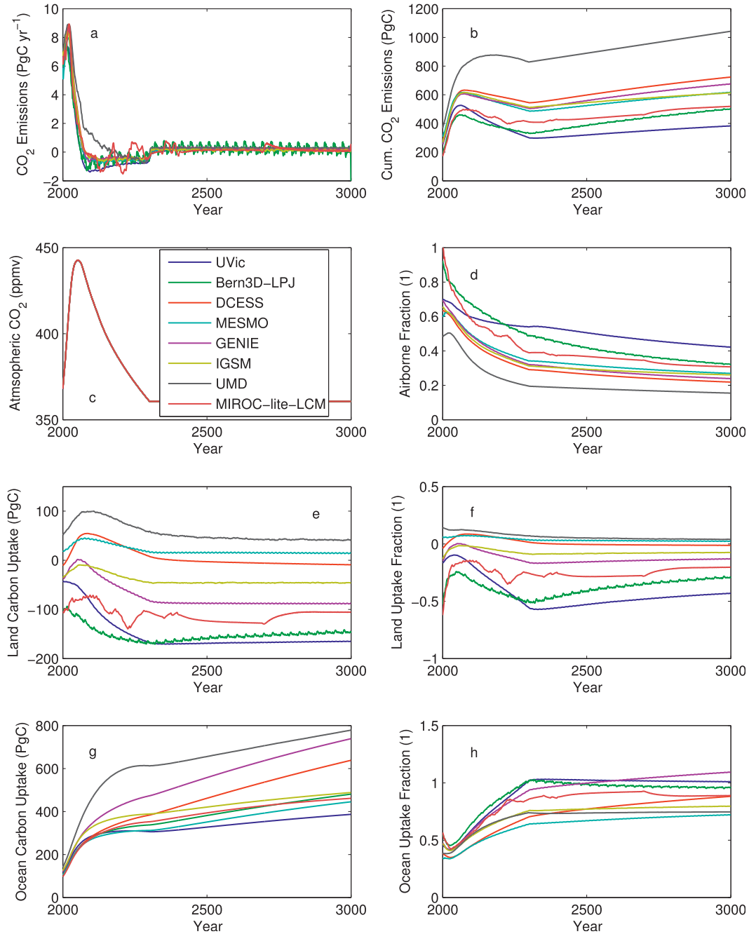
FIG. 4. Changes in carbon inventories in RCP2.6 CCO commitment simulations for eight EMICs with an interactive carbon cycle: (a) CO 2 emissions, (b) cumulative CO 2 emissions since 1850, (c) atmospheric CO 2 concentration, (d) airborne fraction of cumulative emissions, (e) land uptake since 1850, (f) fraction of cumulative emissions taken up by land, (g) ocean uptake since 1850, and (h) fraction of cumulative emissions taken up by ocean. Note that for individual models the ocean uptake fraction can be >1, if the land uptake fraction is <0. Data in (a) were smoothed using a 10-yr moving average.
